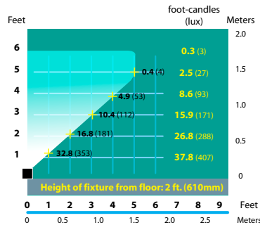
SL-35 Half Spread Photometrics
